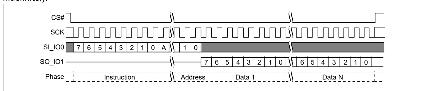
Figure 65 Read command sequence [30]
