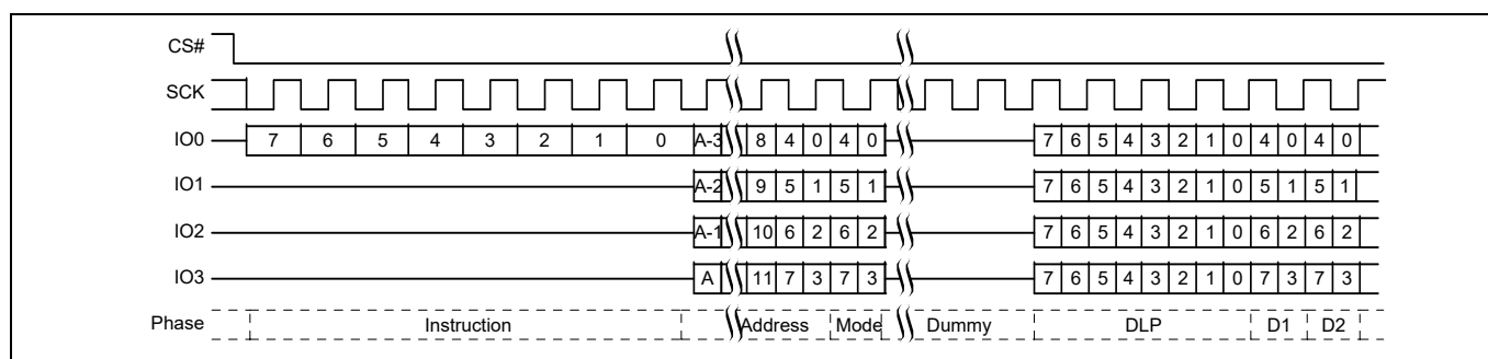
Figure 74 DDR Quad I/O Read initial access [38, 39]
