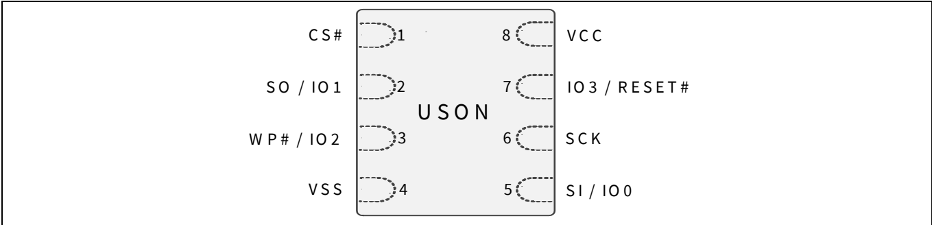
Figure 3 8-pin connector package (USON 4 x 4), top
