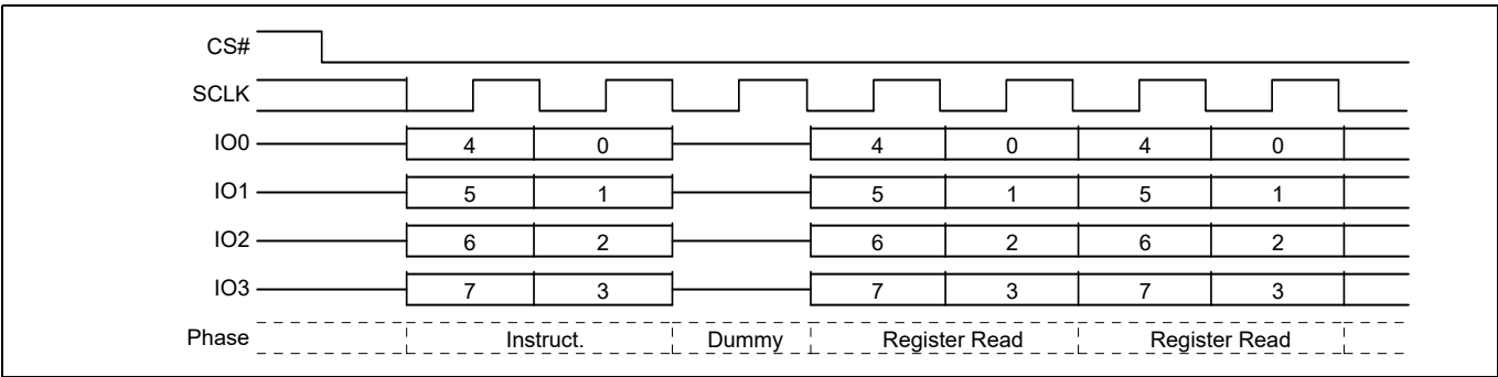
Figure 54 DLPRD Read (DLPRD) command sequence – QPI mode
