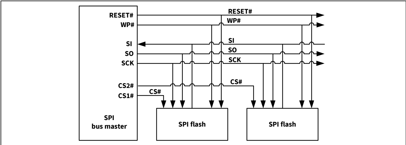
Figure 7 Bus master and memory devices on the SPI bus - Single bit data path
