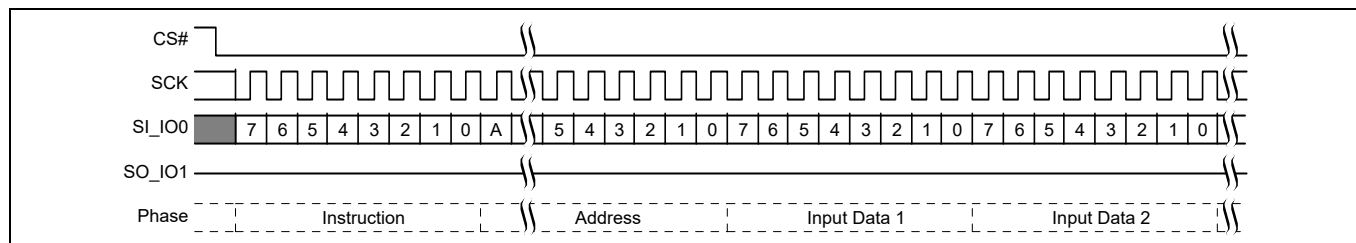
Figure 77 Page Program (PP 02h or 4PP 12h) command sequence [41]
