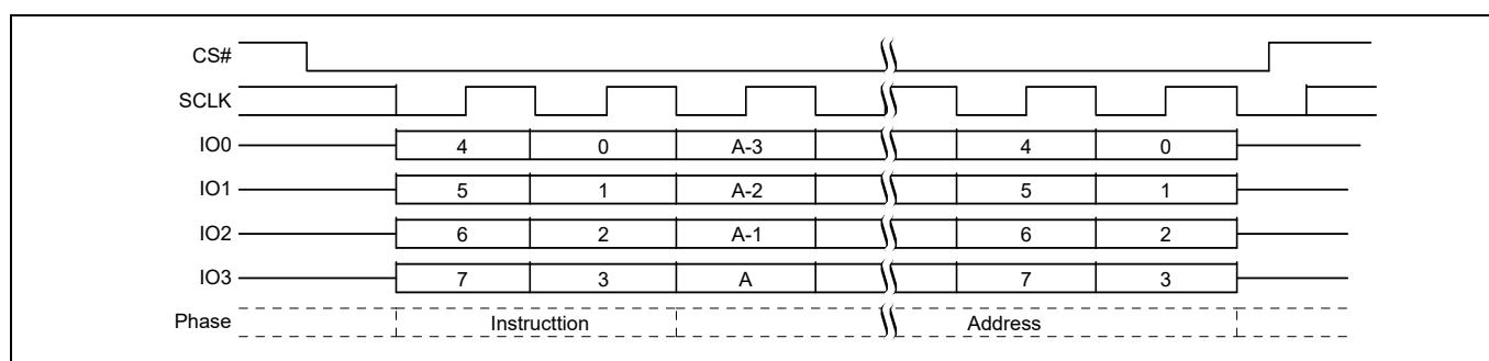
Figure 85 Block Erase (BE D8h or 4BE DCh) QPI mode command sequence [46]
