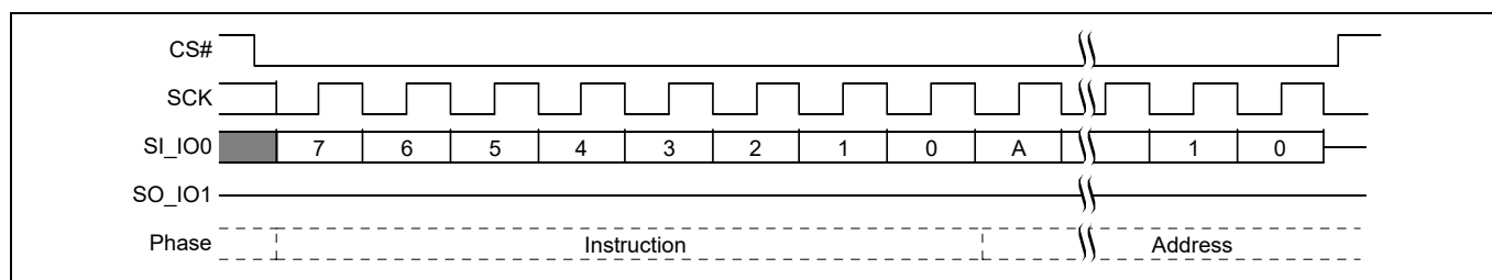
Figure 80 Sector Erase (SE 20h or 4SE 21h) command sequence [43]
