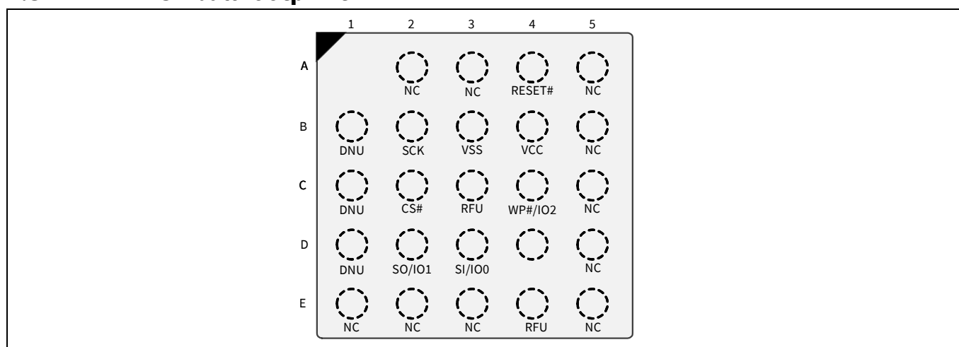
Figure 5 24-ball BGA, 5 x 5 ball footprint (FAB024), top view [4, 5]
