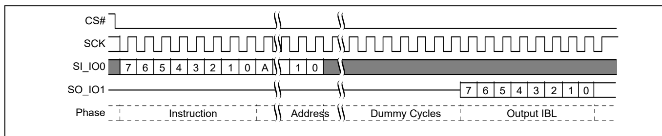
Figure 95 IBLRD command sequence [50, 51]
