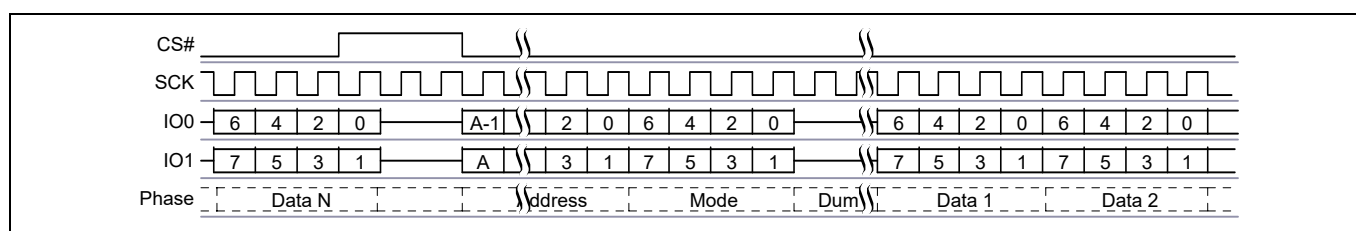
Figure 70 Dual I/O Continuous Read command sequence [33]
