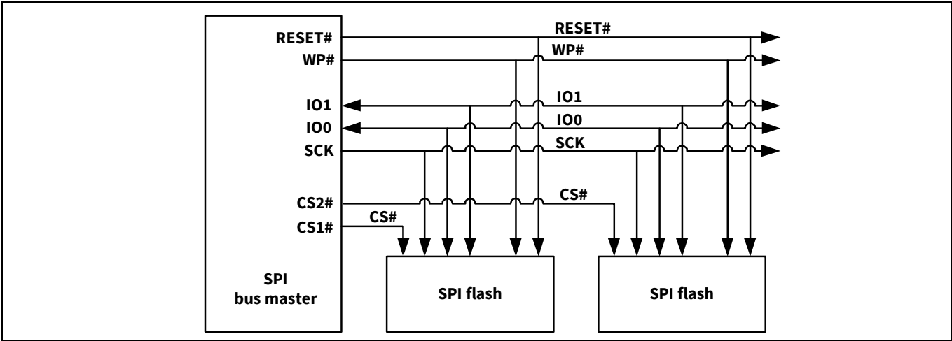
Figure 8 Bus master and memory devices on the SPI bus - Dual bit data path
