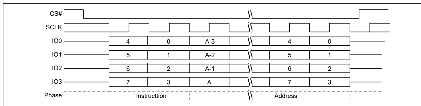
Figure 98 IBL command sequence QPI mode [52, 53]
