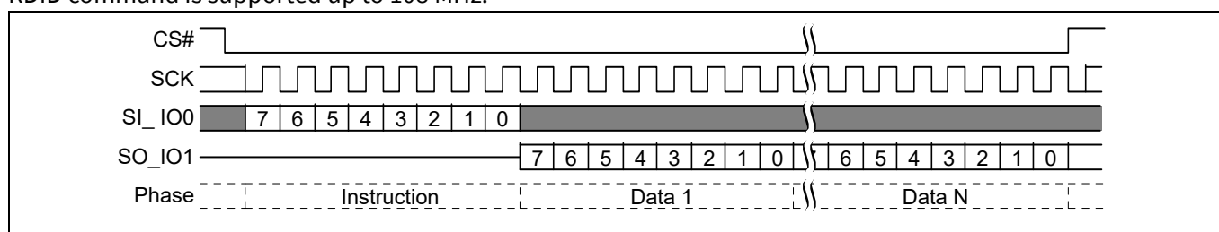
Figure 27 Read Identification (RDID) command sequence
