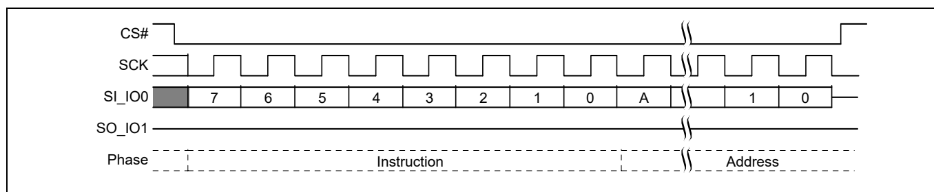
Figure 99 IBUL command sequence [53, 54]
