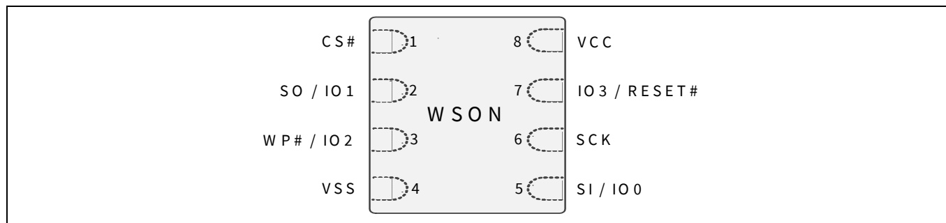
Figure 4 8-connector package (WSO5 5 x 6), top view [3]
