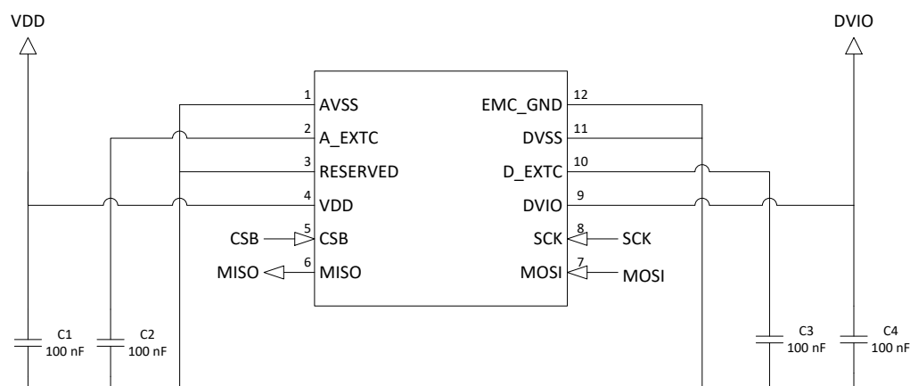
Figure 16 Application schematic.
