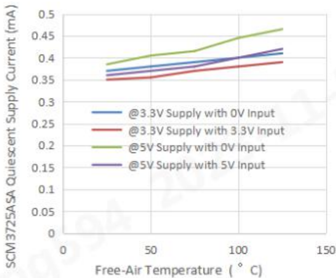
Figure6. SCM3725ASA Quiescent Supply Current vs. Free-Air Temperature
