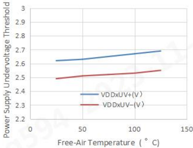
Figure4. UVLO vs. Free-Air Temperature
