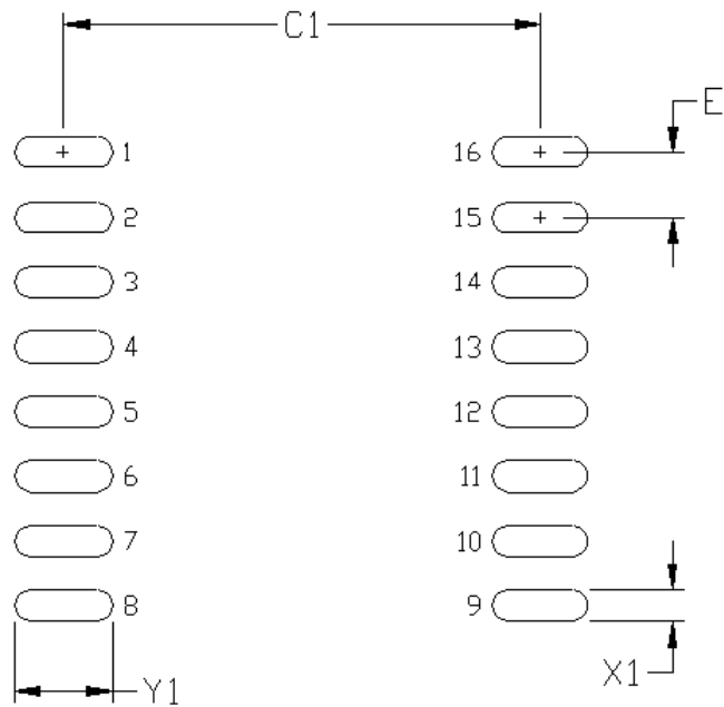
Figure 8.1. 16-Pin SOIC Land Pattern
