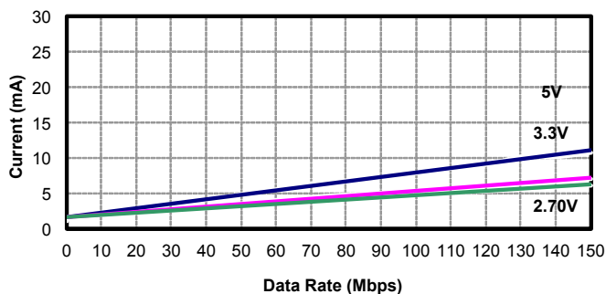
Figure 4.7. Si8422 Typical V_{DD1} or V_{DD2} Supply Current vs. Data Rate 5, 3.3, and 2.70 V Operation (15 pF Load)
