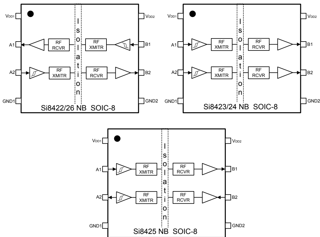
Figure 6.2. Narrow-Body SOIC
