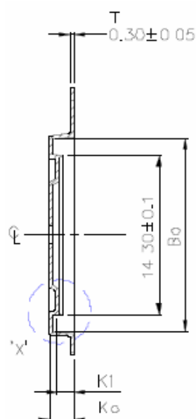
SECTION Y-Y
