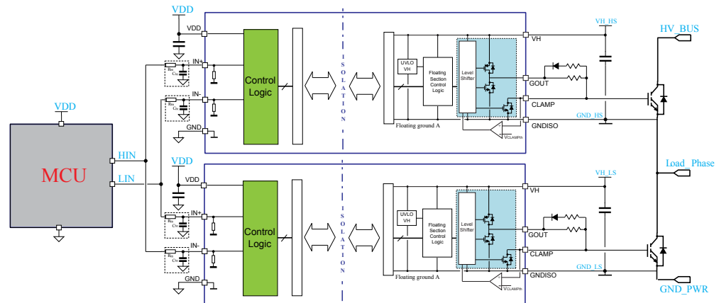
Figure 9. Typical application diagram - Miller clamp
