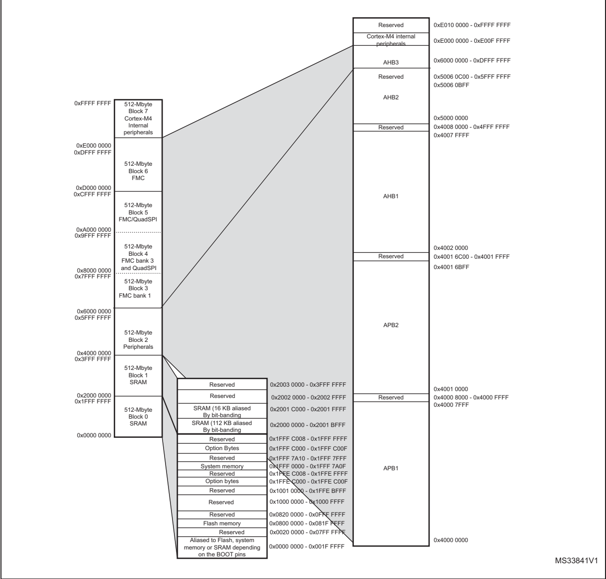
Figure 15. Memory map
