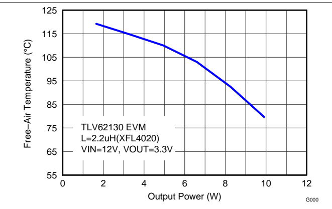
Figure 37. Maximum Ambient Temperature ( F_{SW} = 2.5\text{ MHz} )
