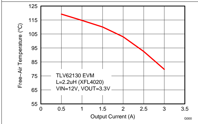
Figure 36. Maximum Ambient Temperature ( F_{SW} = 2.5\text{ MHz} )
