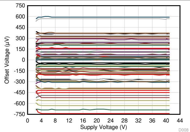
Figure 6-6. Offset Voltage vs Power Supply
