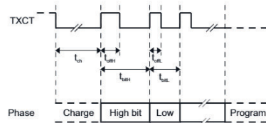
Figure 5-5. Transponder Write Protocol
