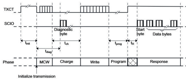
Figure 5-3. Write/Read Mode (Writing Into Mode Control Register)
