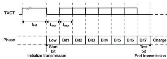
Figure 5-4. Mode Control Write Protocol (NRZ Coding)
