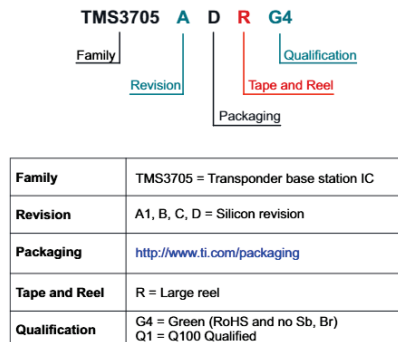
Figure 8-1. Device Nomenclature
