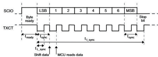
Figure 5-7. Transmission on SCIO in Synchronous Mode (NRZ Coding) (For Diagnosis Byte and Data Bytes)
