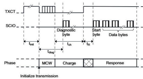
Figure 5-2. Read-Only Mode (Writing Into Mode Control Register)
