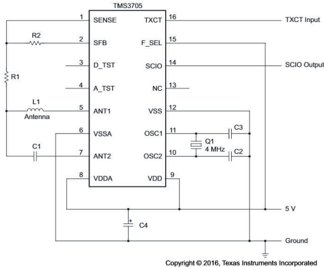
Figure 7-1. Application Diagram
