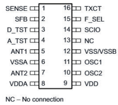
Figure 4-1. 16-Pin D Package (Top View)
