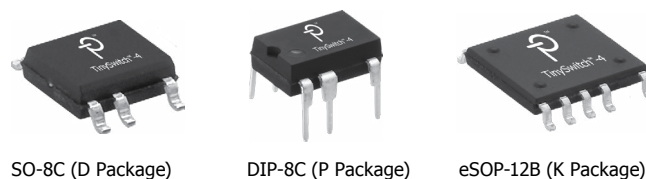
Figure 2. Package Options.
