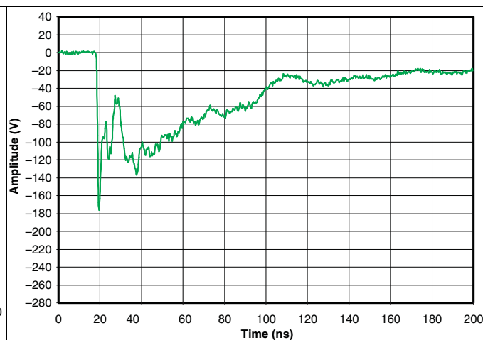
Figure 2. -8-kV Contact
