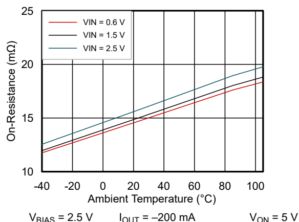
Figure 6-10. On-Resistance vs Ambient Temperature Single Channel (TPS22976)
