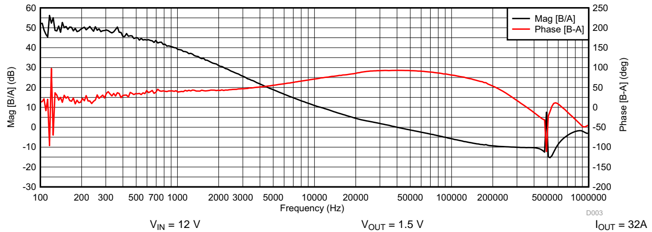
Figure 62. Bode Plot
