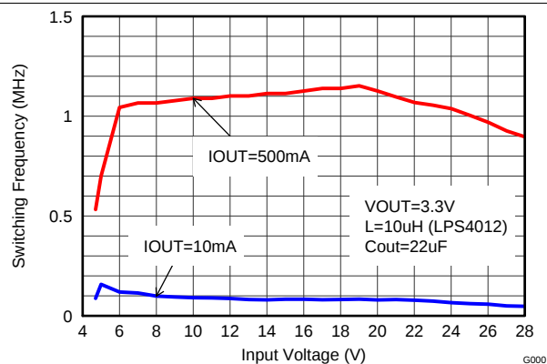
Figure 28. Switching Frequency
