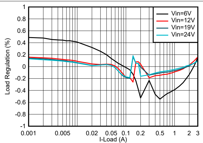
Figure 10-3. Load Regulation
