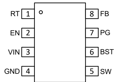
Figure 7-2. TPS62933P and TPS62933O 8-Pin SOT583 DRL Package (Top View)
