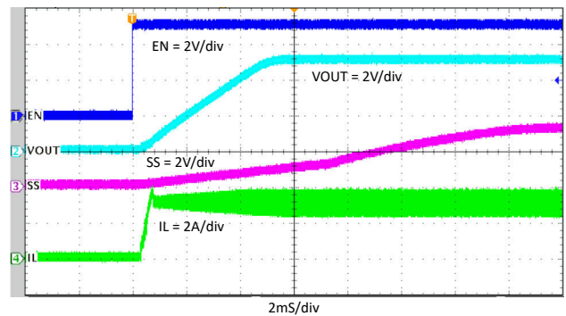
Figure 10-11. Start-Up Through EN, I_{OUT} = 3\text{ A}
