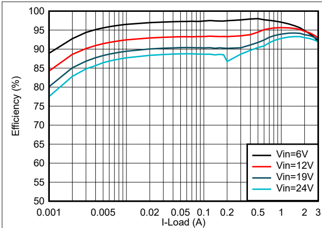
Figure 10-2. Efficiency
