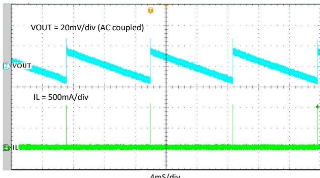
Figure 10-13. Steady State, I_{OUT} = 0\text{ A}
