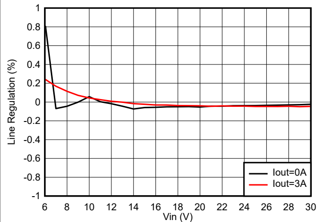
Figure 8-34. TPS62933O Line Regulation, V_{OUT} = 5\text{ V} , f_{SW} = 500\text{ kHz}
