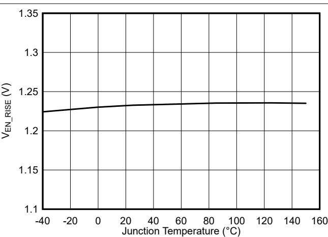
Figure 8-6. Enable Threshold vs Junction Temperature
