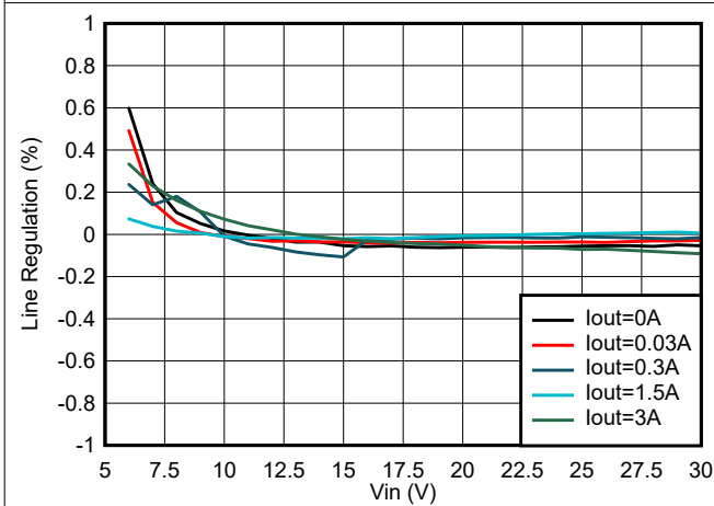
Figure 10-4. Line Regulation
