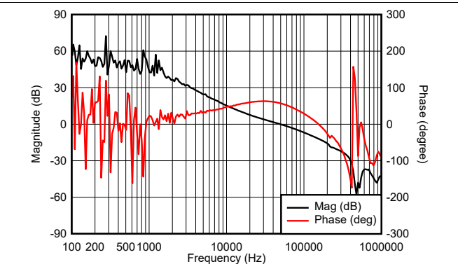
Figure 10-7. Loop Frequency Response, I_{OUT} = 3\text{ A} , BW = 49.4\text{ kHz} , PM = 57^\circ , GM = -12\text{ dB}
