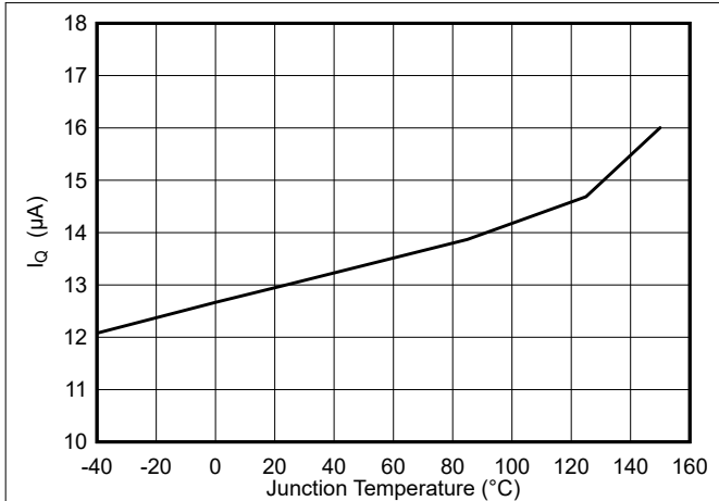
Figure 8-1. TPS62933 Quiescent Current vs Junction Temperature
