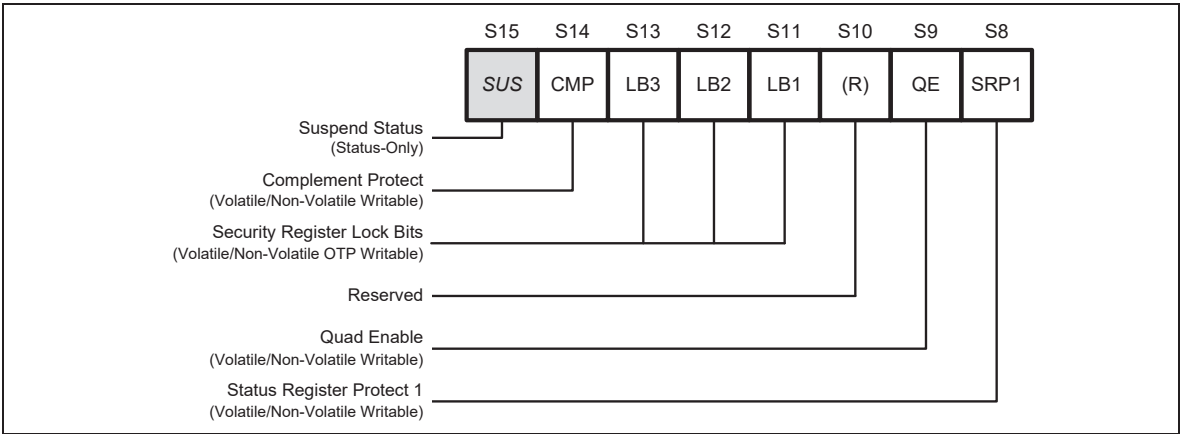
Figure3b. Status Register-2
