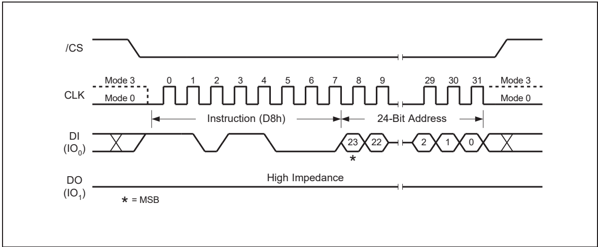
Figure 23. 64KB Block Erase Instruction Sequence Diagram
