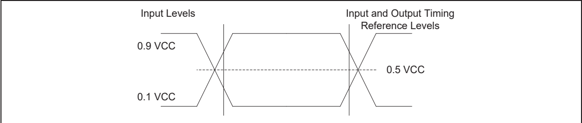
AC Measurement I/O Waveform
