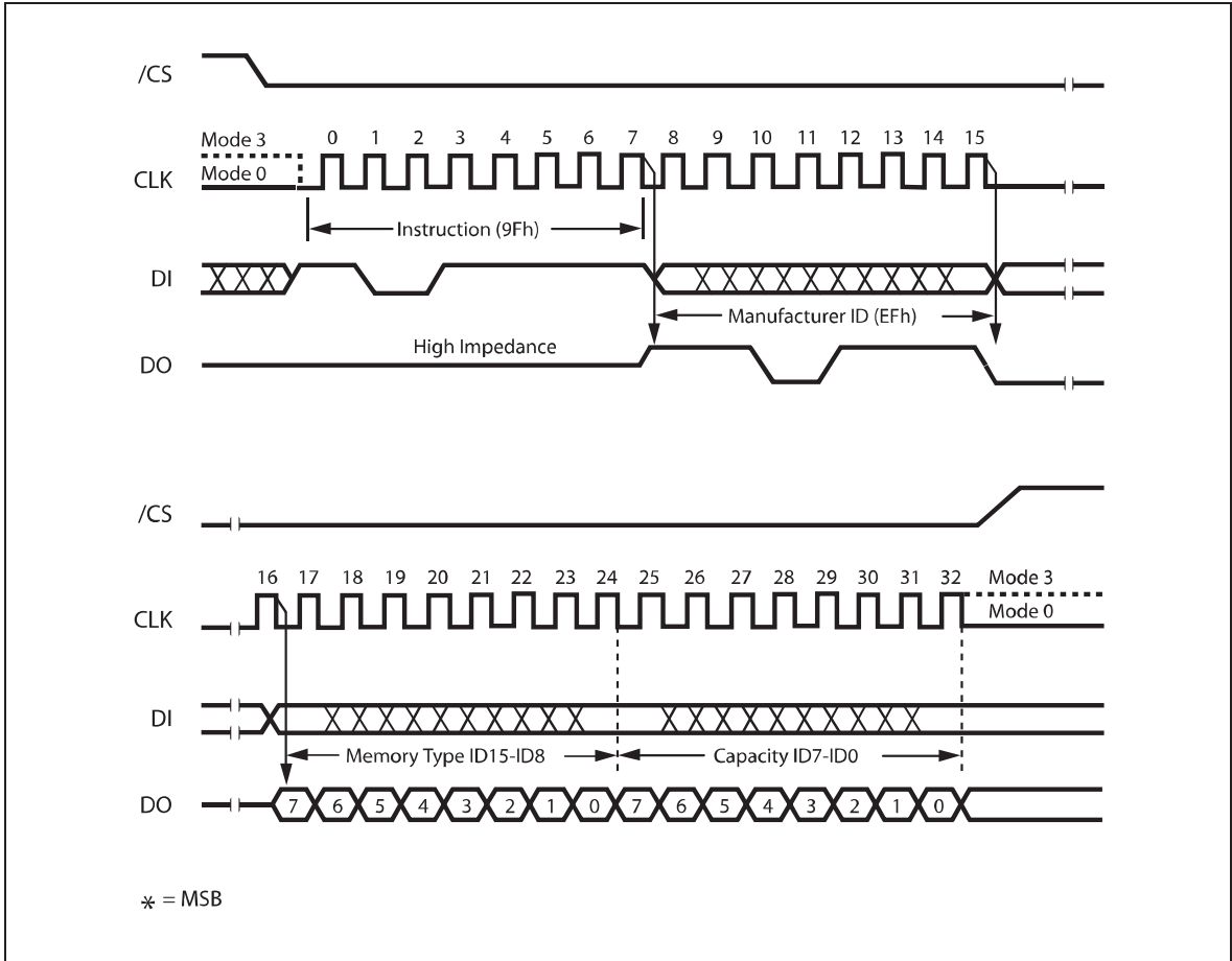
Figure 33a. Read JEDEC ID Instruction Sequence
