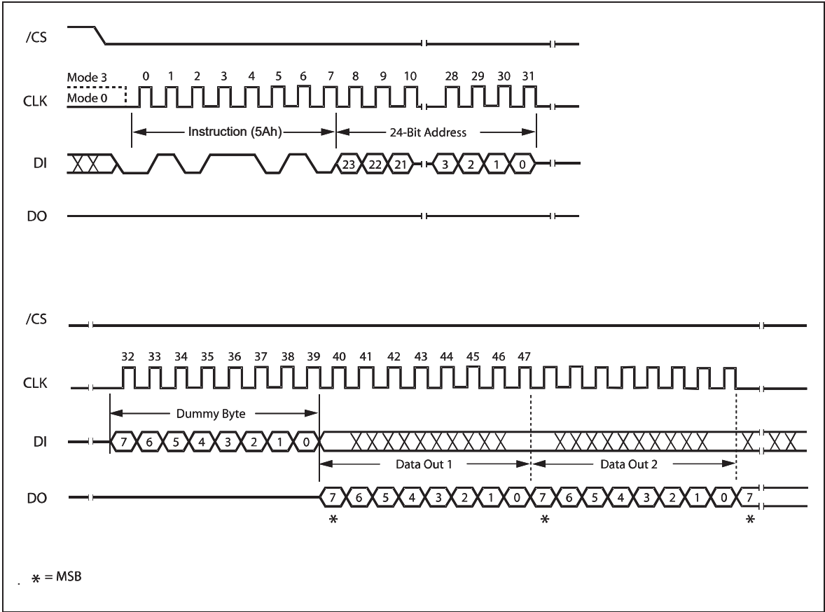
Figure 34b. Read SFDP Register Instruction Sequence Diagram
