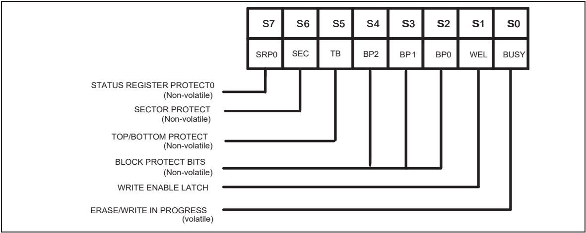
Figure3a. Status Register-1
