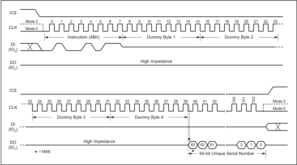
Figure 32. Read Unique ID Number Instruction Sequence
