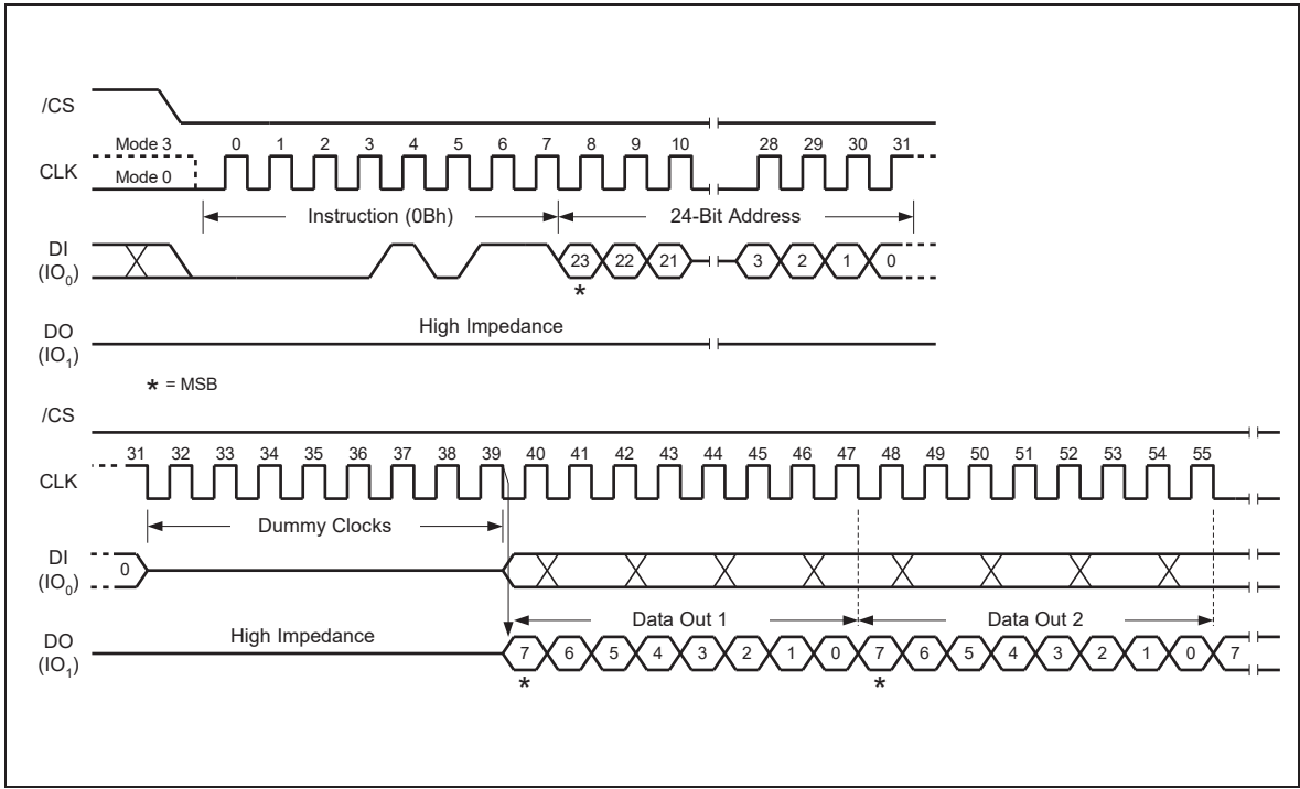
Figure 10. Fast Read Instruction Sequence Diagram
