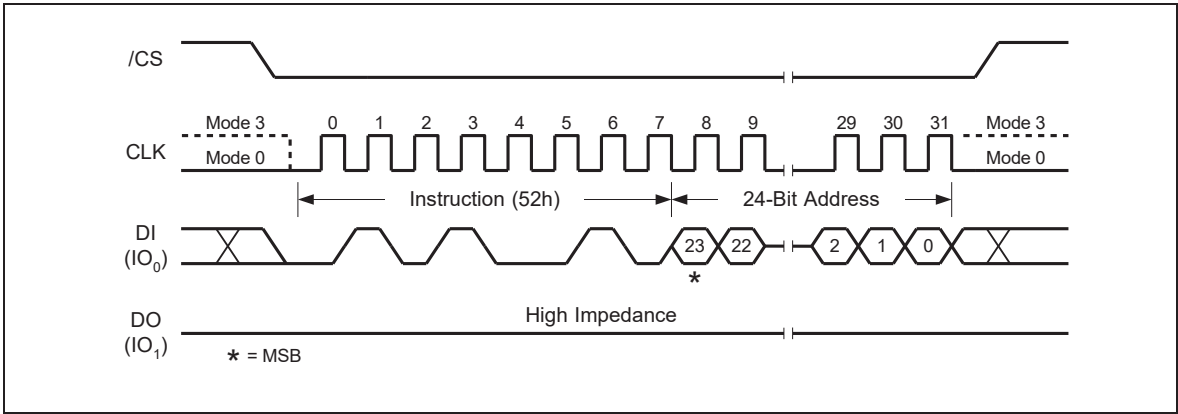
Figure 22a. 32KB Block Erase Instruction Sequence Diagram
