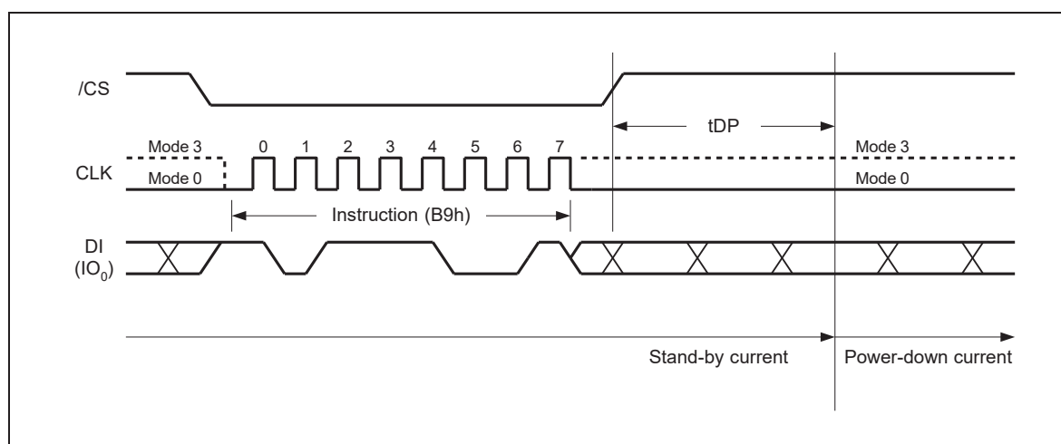
Figure 27. Deep Power-down Instruction Sequence Diagram
