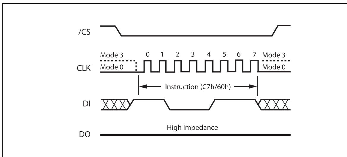
Figure 24. Chip Erase Instruction
