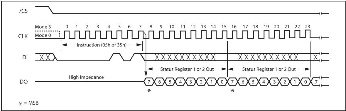
Figure 7. Read Status Register Instruction Sequence Diagram
