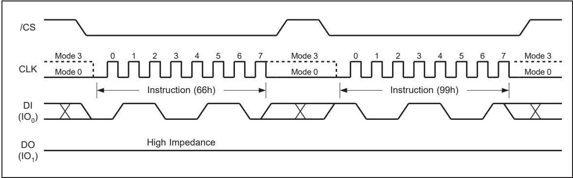
Figure 39a. Enable Reset and Reset Instruction Sequence
