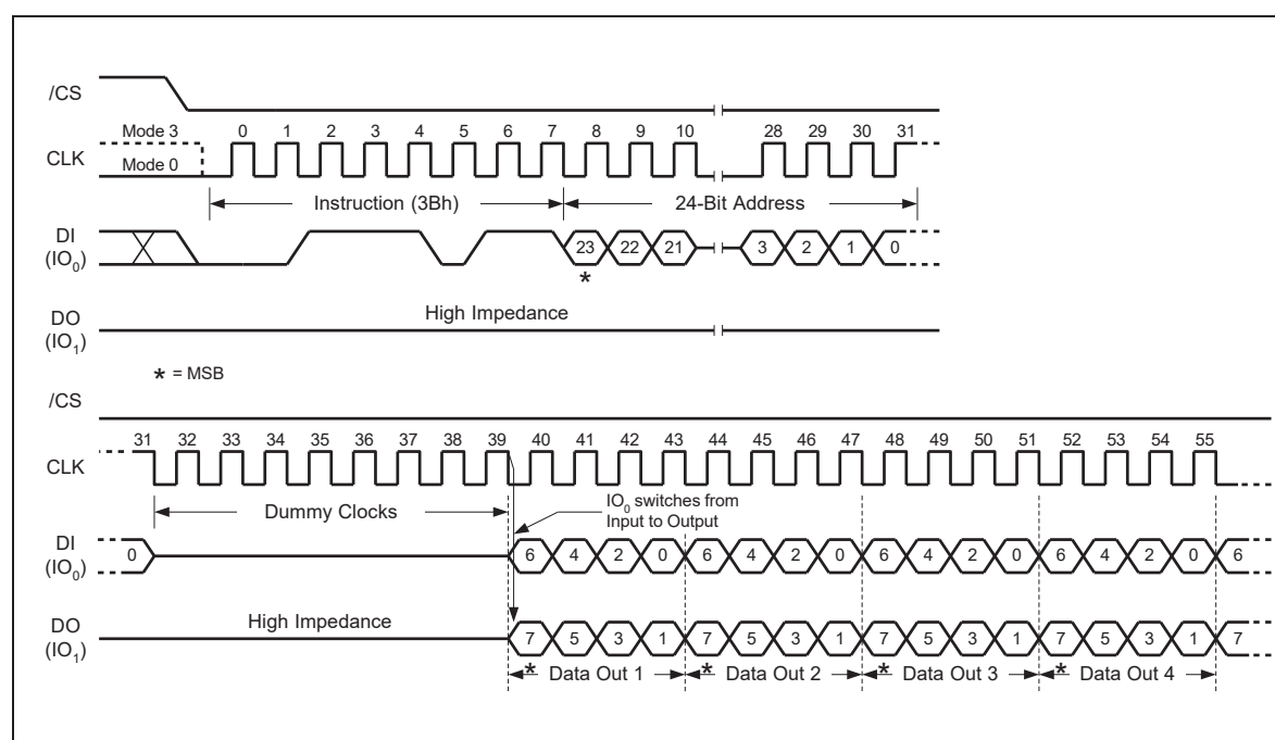
Figure 11. Fast Read Dual Output Instruction Sequence Diagram
