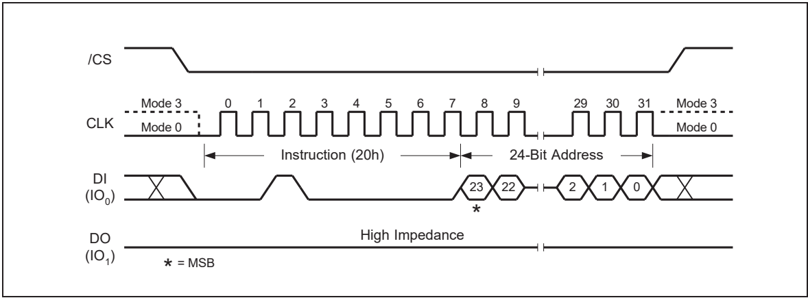
Figure 21a. Sector Erase Instruction Sequence Diagram
