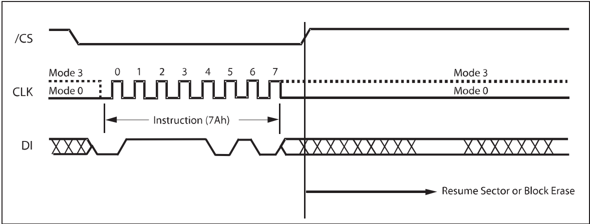
Figure 26a. Erase/Program Resume Instruction Sequence
