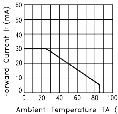
Fig.3 FORWARD CURRENT DERRATING CURVE
