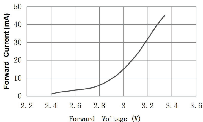
伏安特性曲线 Forward Current VS. Forward Voltage ( T_a=25^\circ\text{C} )
