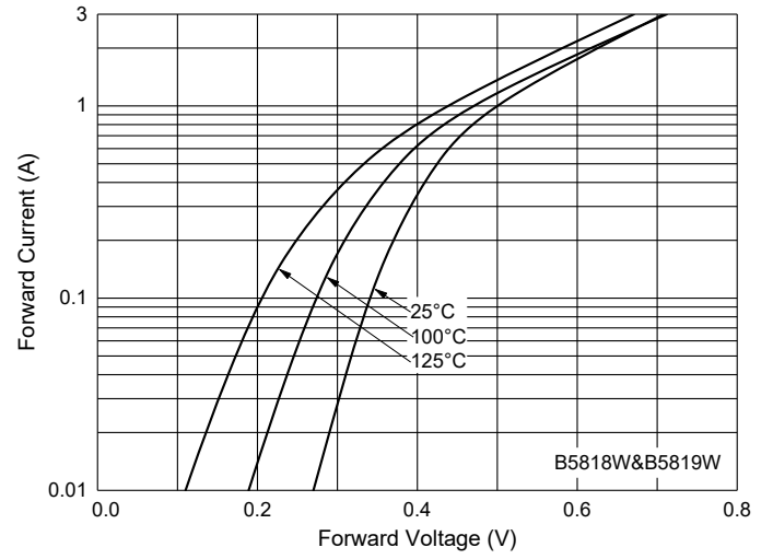
Fig. 2 - Forward Characteristics
