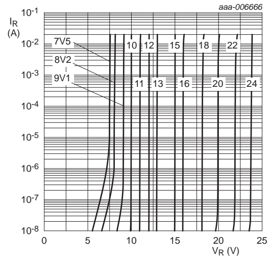
BZX384-B/C7V5 to BZX384-B/C24 T_{amb} = 25\text{ °C}
