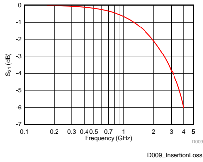
Figure 11. Insertion Loss
