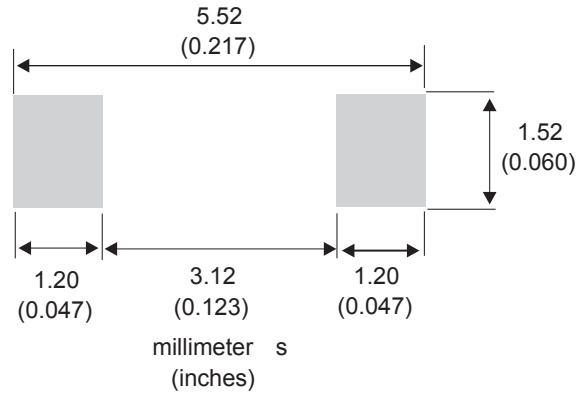
Figure 19. SMA Flat recommended footprint in mm (inches)
