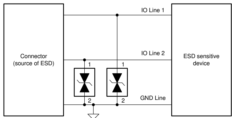
Application Schematic
