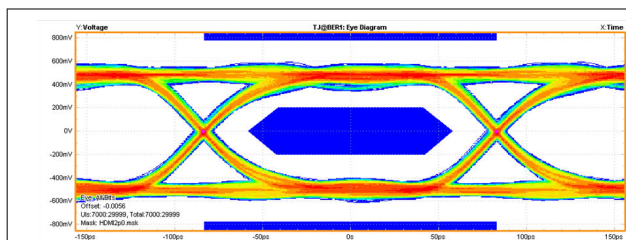
Figure 8-8. 6-Gbps HDMI 2.0 (TP1) Eye Diagram TPD4E05U06
