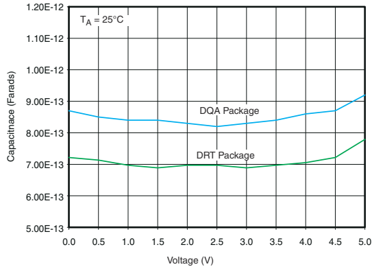
Figure 6-1. IO Capacitance vs IO Voltage
