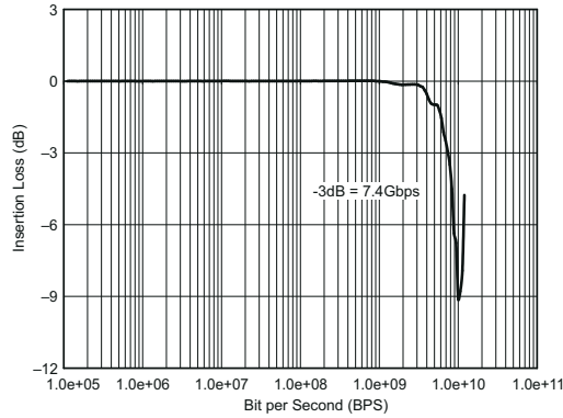
Figure 6-7. Insertion Loss
