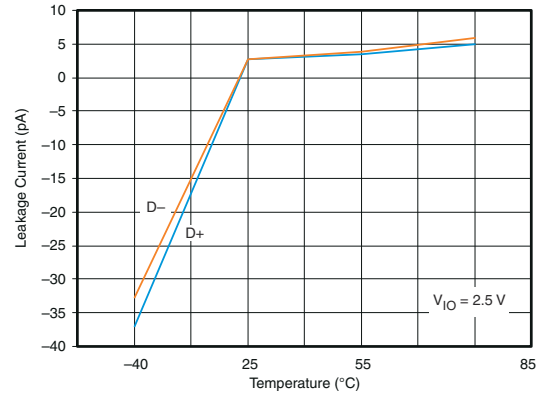
Figure 6-2. Leakage Current vs Temperature
