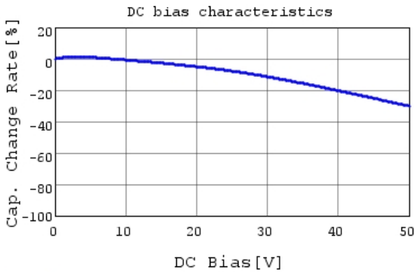
GCM188R71H103KA37 C-DC bias capchange, 25.0c
