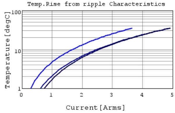
GRM188R61E106MA73 Temp.rise — 80kHz —
