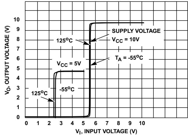
Figure 6-8. Typical Voltage Transfer Characteristics as a Function of Temperature for CD4050B
