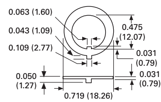
Locking Ring
