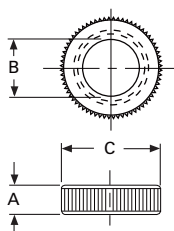
Knurled Dress Nut Catalog No. 15-1048-3
