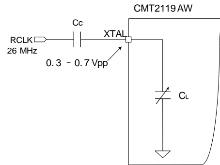
Figure 15. RCLK Circuitry
