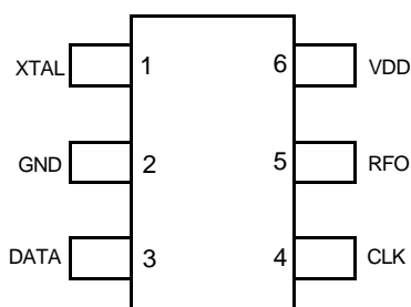
Figure 2. CMT2119AW Pin Assignments
