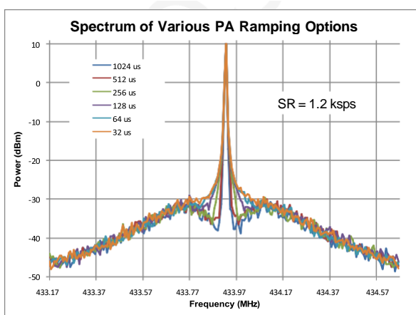
Figure 7. Spectrum of PA Ramping, SR = 1.2 ksps, P_{OUT} = +10 dBm
