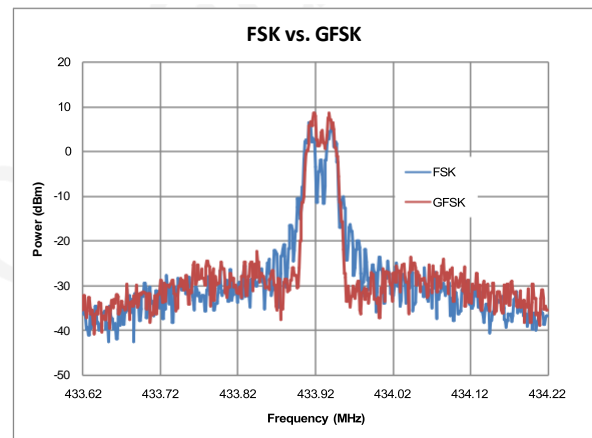
Figure 6. FSK/GFSK Spectrum, SR = 9.6 ksps, F_{DEV} = 15 kHz
