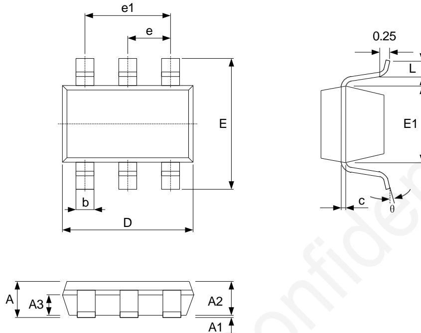
Figure 24. 6-Pin SOT23-6
