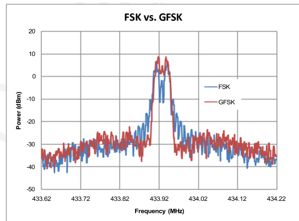
Figure 6. FSK/GFSK Spectrum, SR = 9.6 ksps, F_{DEV} = 15 kHz
