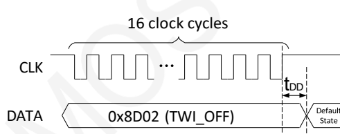
Figure 22. TWI_OFF Command
