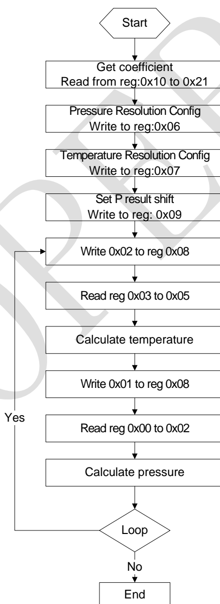
Figure 10: flow chart
