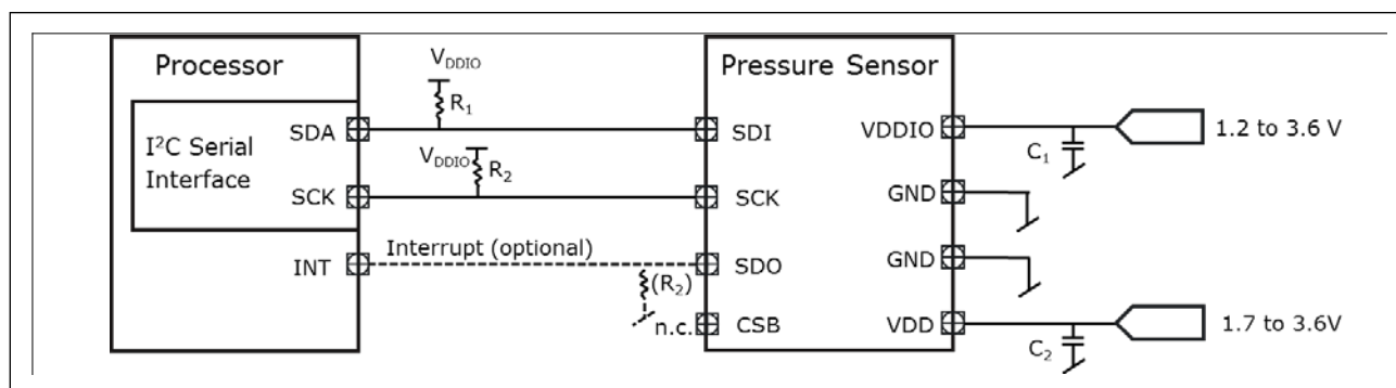
Figure4: Application Circuit Example using the SPI 4-wires serial interface
