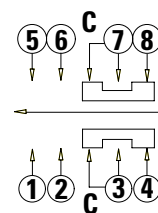
Circuit Diagram C: Common Pin Bottom View
