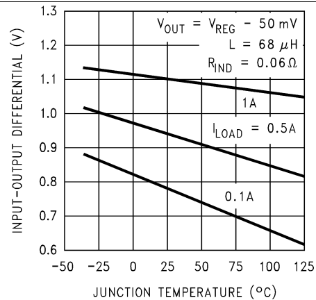
Figure 6. Dropout Voltage
