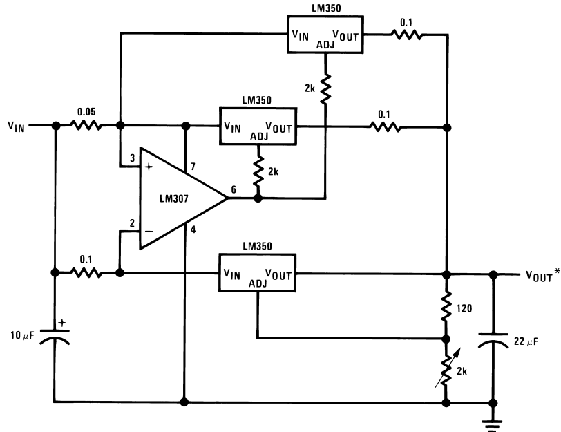
Figure 26. 10A Regulator
