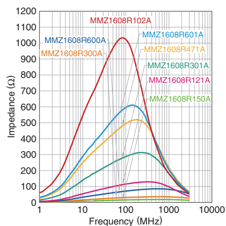
MMZ1608R series
