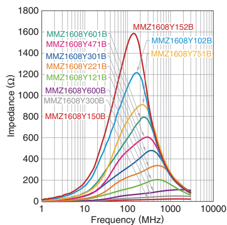
MMZ1608Y series
