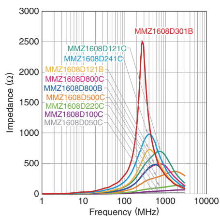
MMZ1608D series
