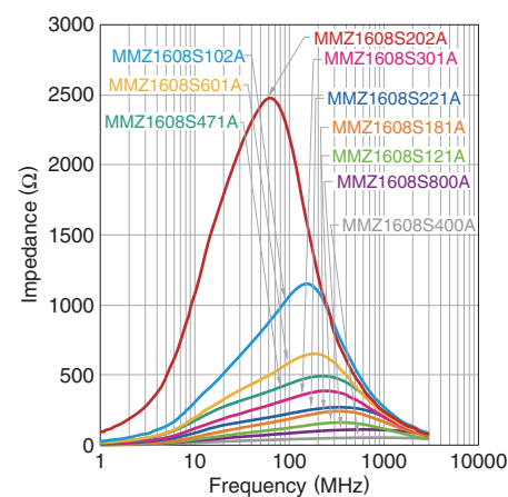
MMZ1608S series
