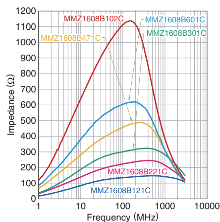
MMZ1608B series
