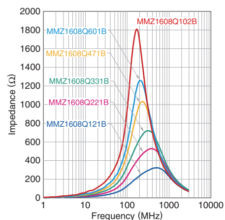
MMZ1608Q series
