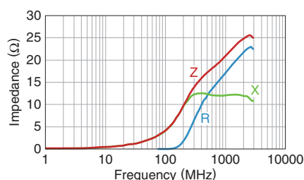
MMZ1608D500CTAH0
