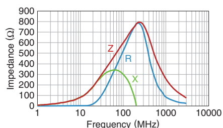
MMZ1608Y601BTA00
