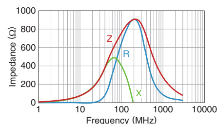
MMZ1608Y751BTA00
