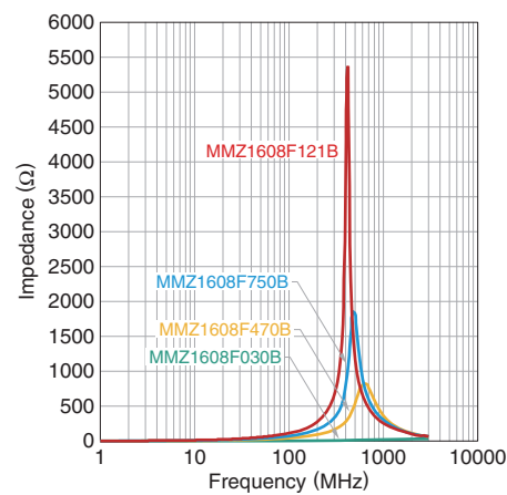
MMZ1608F series
