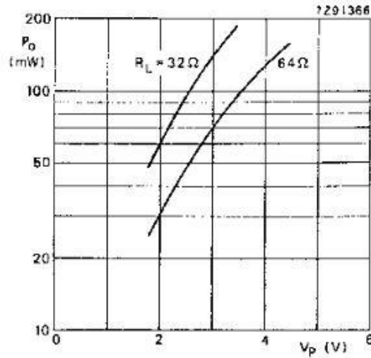
Fig. 2 Output power across the load impedance ( R_L ) as a function of supply voltage ( V_p ) in BTL application. Measurements were made at f = 1 kHz; d_{int} = 10\% ; T_{amb} = 25 °C.
