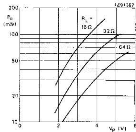
Fig. 3 Output power across the load impedance ( R_L ) as a function of supply voltage ( V_p ) in stereo application. Measurements were made at f = 1 kHz; d_{int} = 10\% ; T_{amb} = 25 °C.
