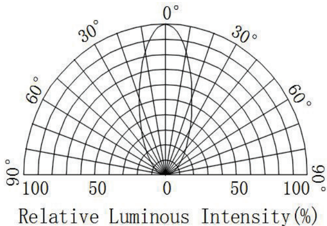
角度图/Directivity Diagram
