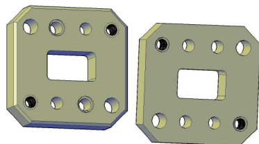
COVER FLANGE (THRU TYPE)
