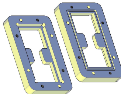
GASKET FLANGE (SOCKET TYPE)
