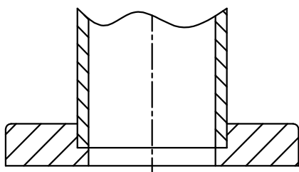
Butt Type, Socket
